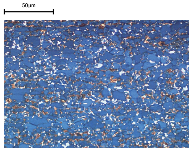
Structural example of cold-rolled DP steels. Microstructural contrasting with color etching according to Klemm.
