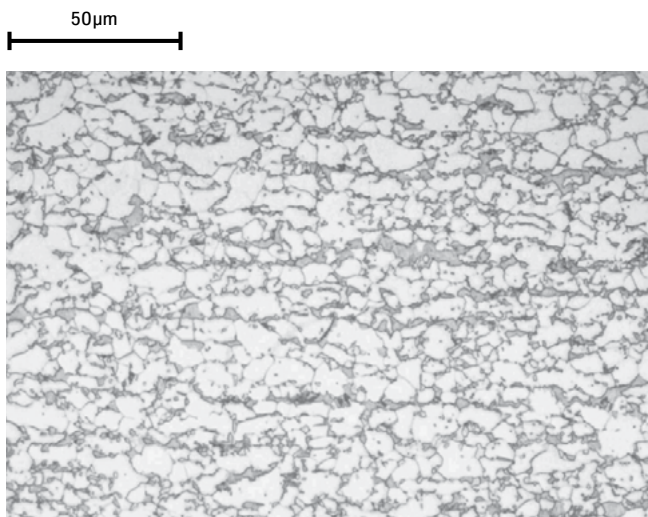
Structural example of cold-rolled DP steels. Microstructural contrasting through etching with nital.
